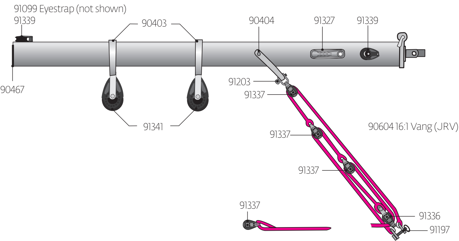
17651 Collegiate 420 Complete Boom
