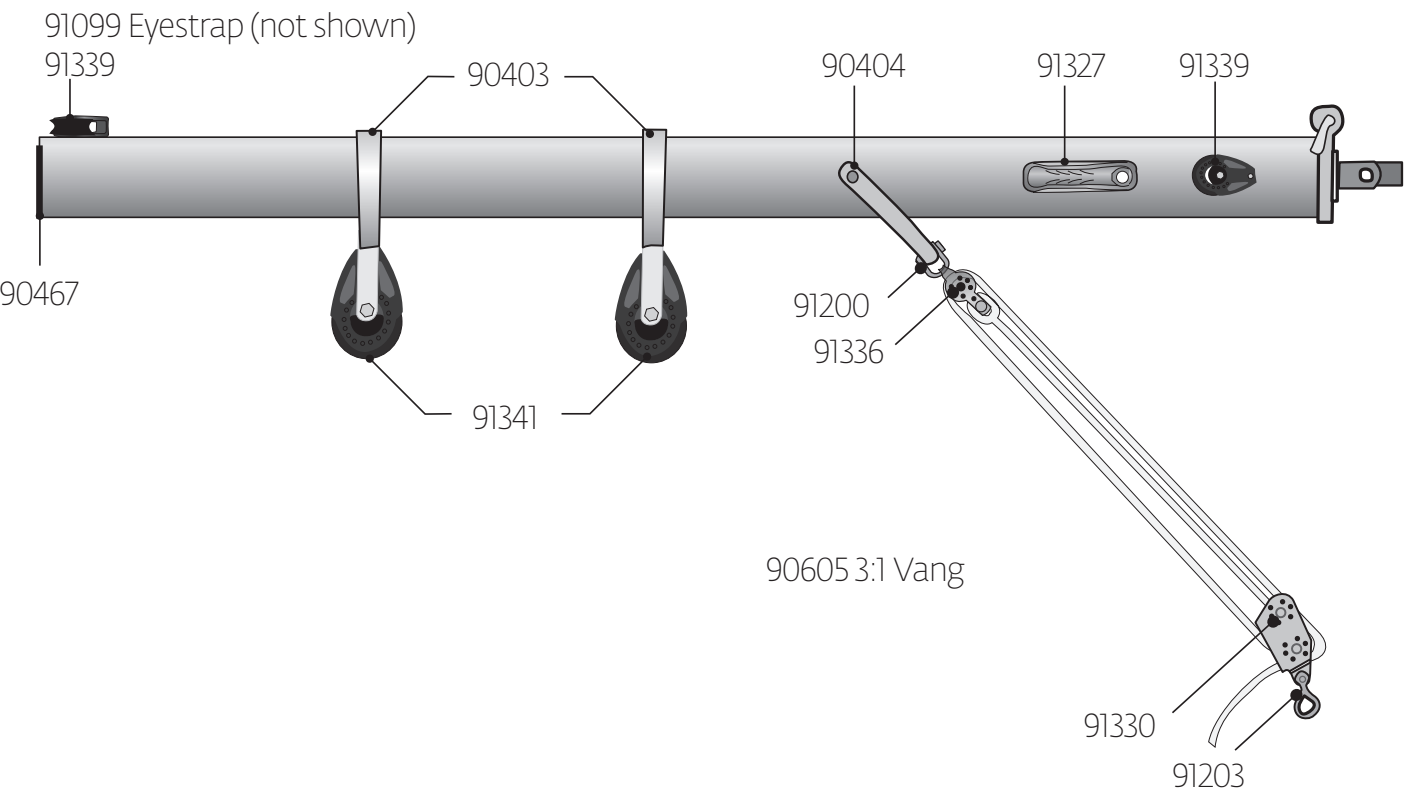
17651 Collegiate 420 Complete Boom
